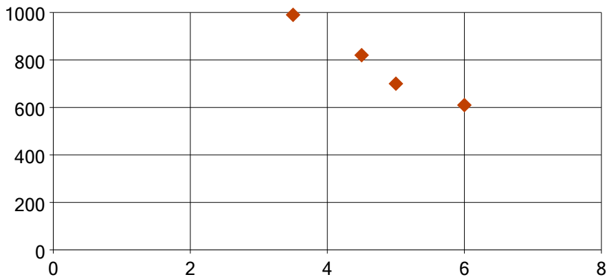
Units sold against price
